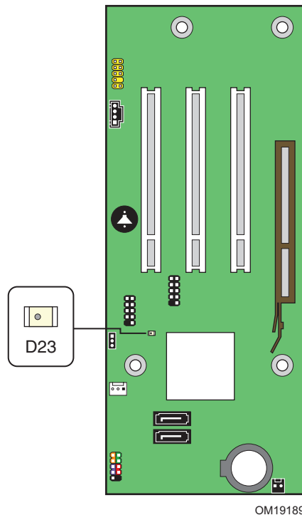
Figure 3. Location of Standby Power Indicator
